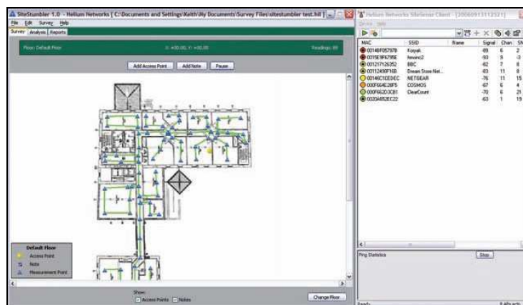
SiteStumbler lets you collect wireless information in real-time.
